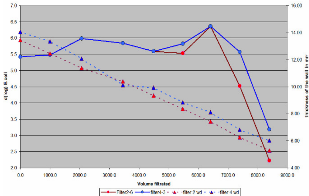
Figure 1: Removal of E.coli and wall thickness of silver-impregnated filters
